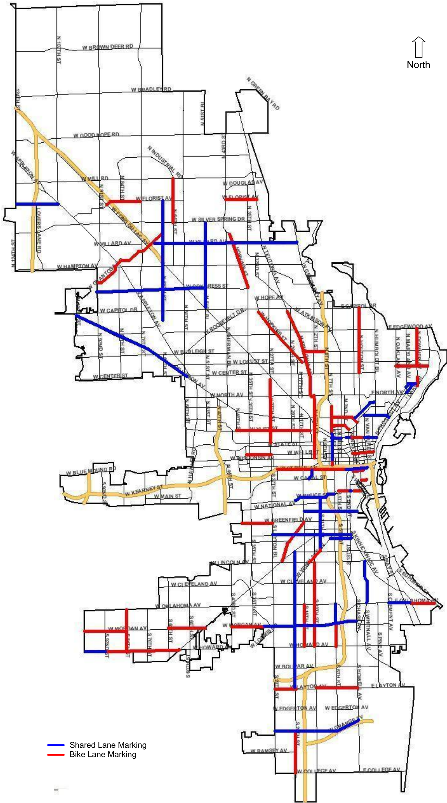
PROJECT 2984-41-00 BICYCLE LANE DELINEATION (NON-HWY) VARIOUS ROADWAYS PAVEMENT MARKINGS 2012 CMAQ PROJECT 60% DESIGN MAP
